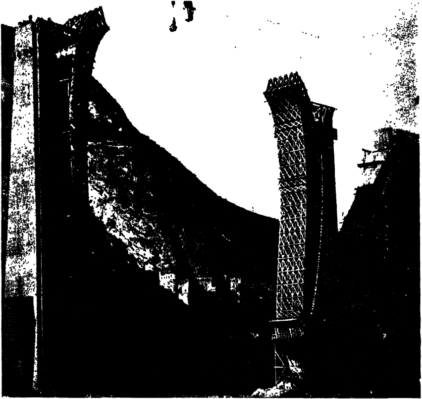
Fig. 298.—Arch Centering Ready for Lowering.
